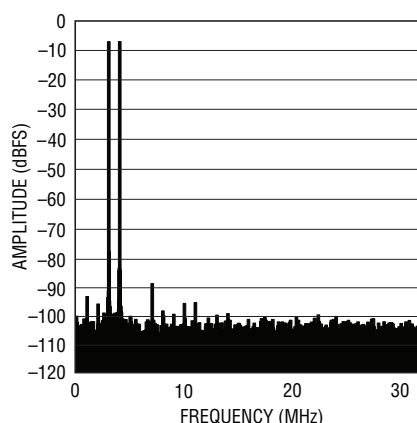
LTC2265-14, 65Msps, 2-Tone FFT, f_{IN} = 70MHz and 75MHz
